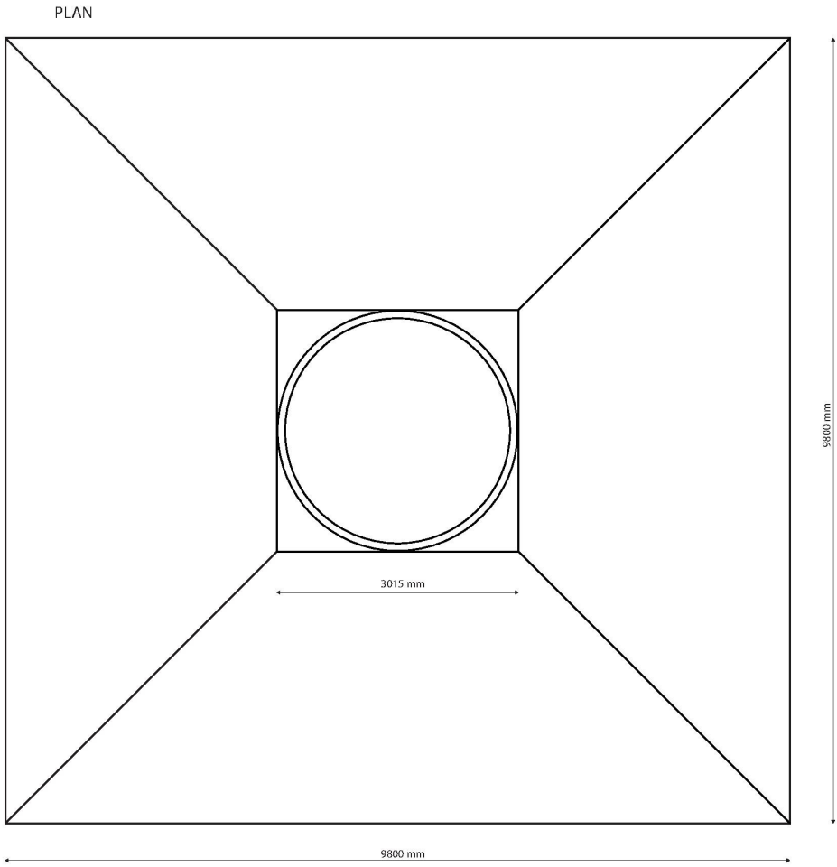
Vestas V47 Foundation Drawing Scale 50:1 at A3
